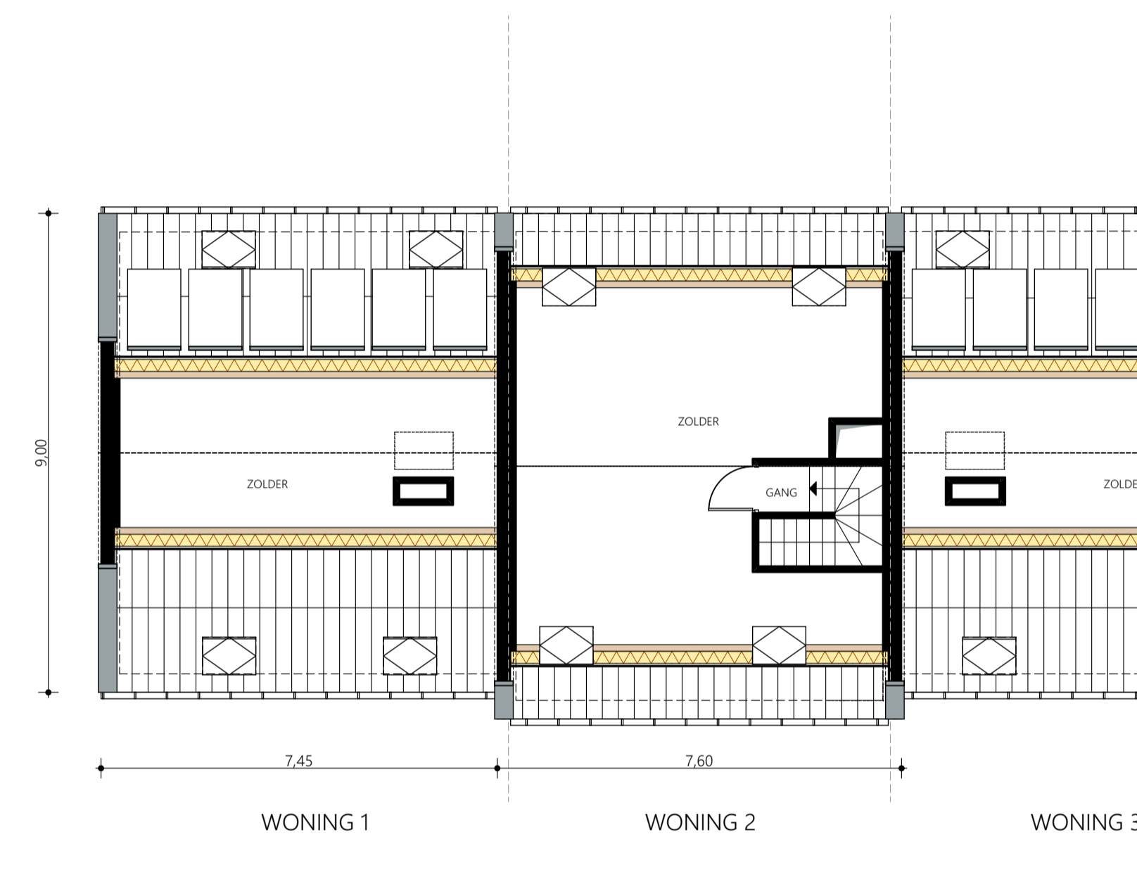
ZOLDERVERDIEPING
